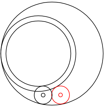
Top View of 2 7/8" EUE Coupling Inside 5 1/2" Casing With 7/8" Cable Head
