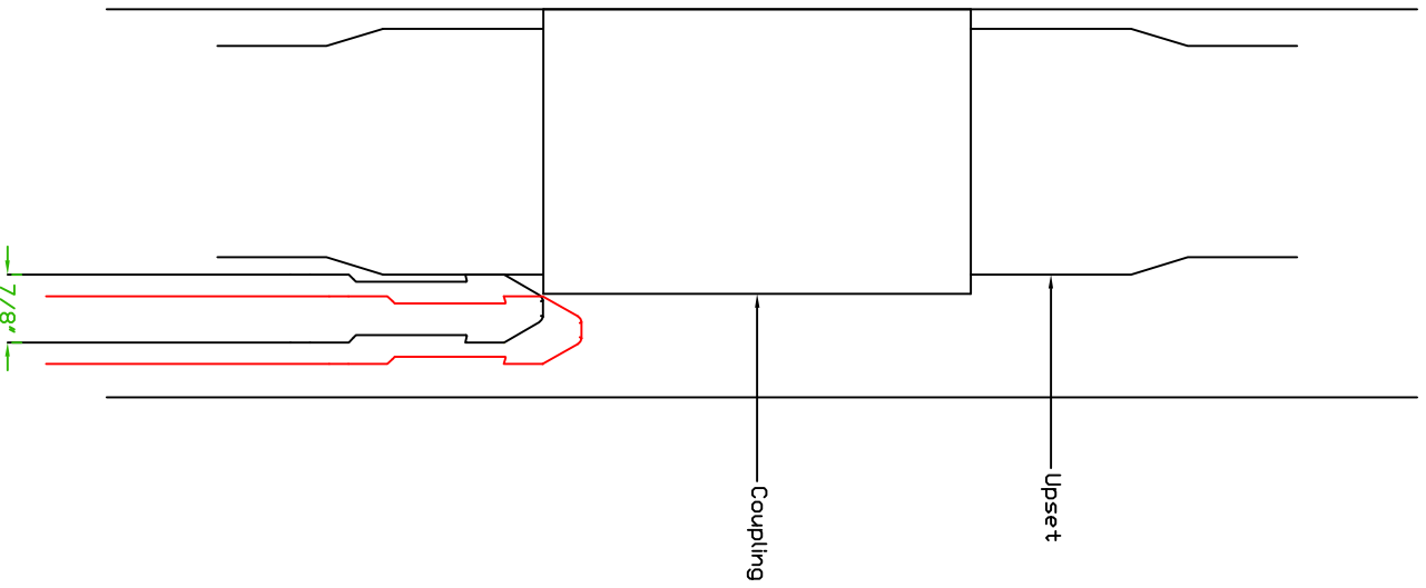
Side View of 7/8" Rope Socket shown clearing 2 7/8" EUE Coupling
