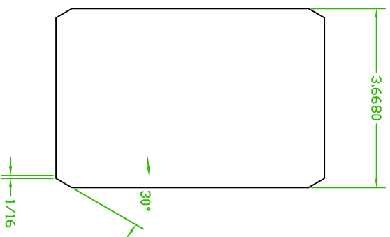
2 7/8" Coupling with 30 degree bevels
