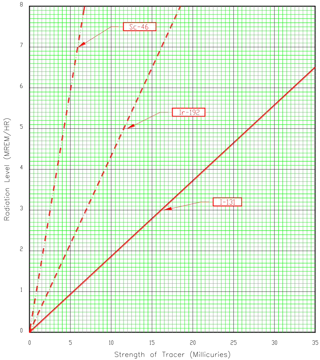
CHART 3 – RADIATION LEVELS AT THREE FEET FROM UNSHIELDED RADIOACTIVE TRACERS
