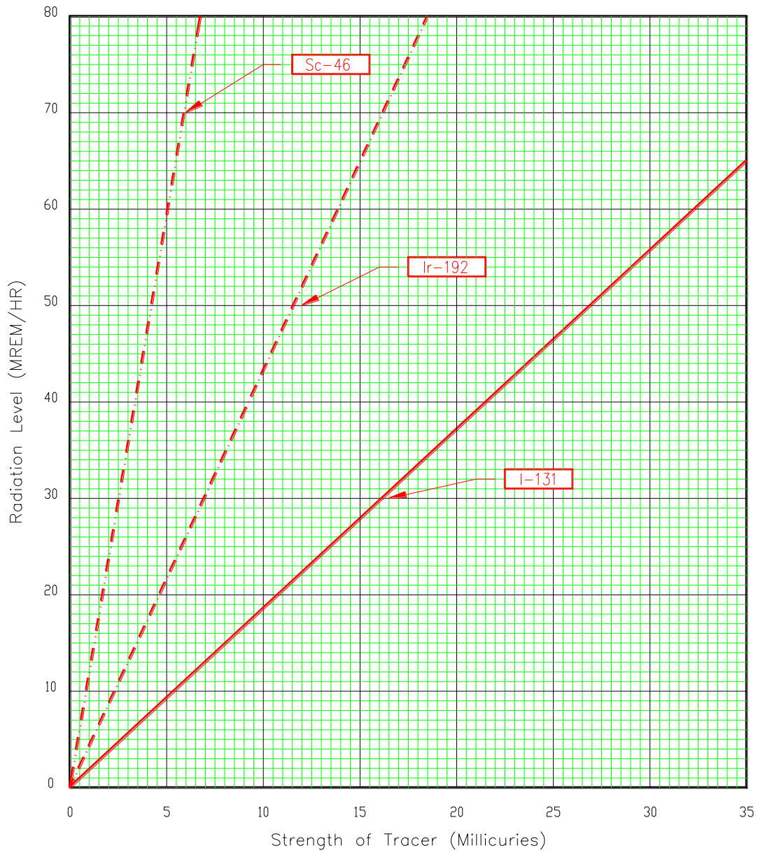
CHART 2 – RADIATION LEVELS AT ONE FOOT FROM UNSHIELDED RADIOACTIVE TRACERS
