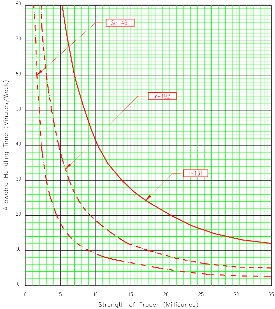
CHART 1 – HAND EXPOSURE FROM RADIOACTIVE TRACERS
